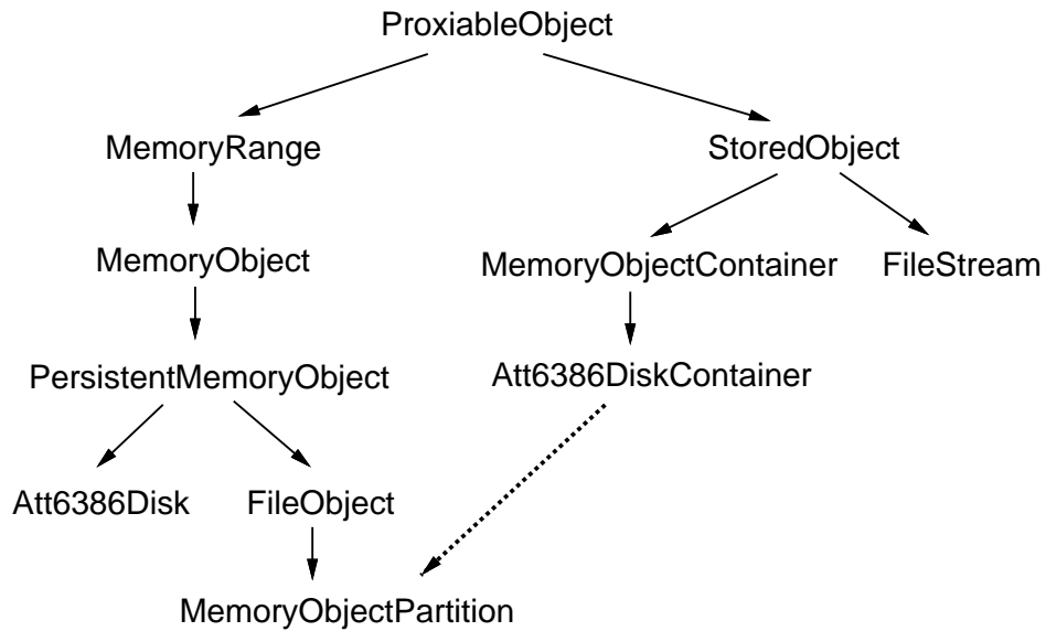
Figure 6.1: Portion of Original Class Hierarchy
