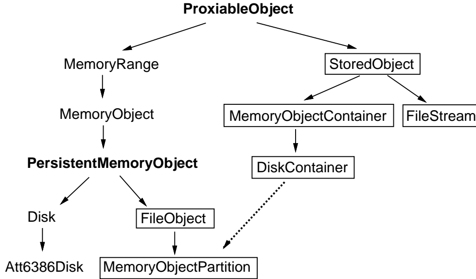
Figure 6.2: Split Class Hierarchy
